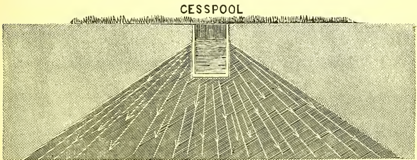
FIG. 12.—Cone of pollution.
